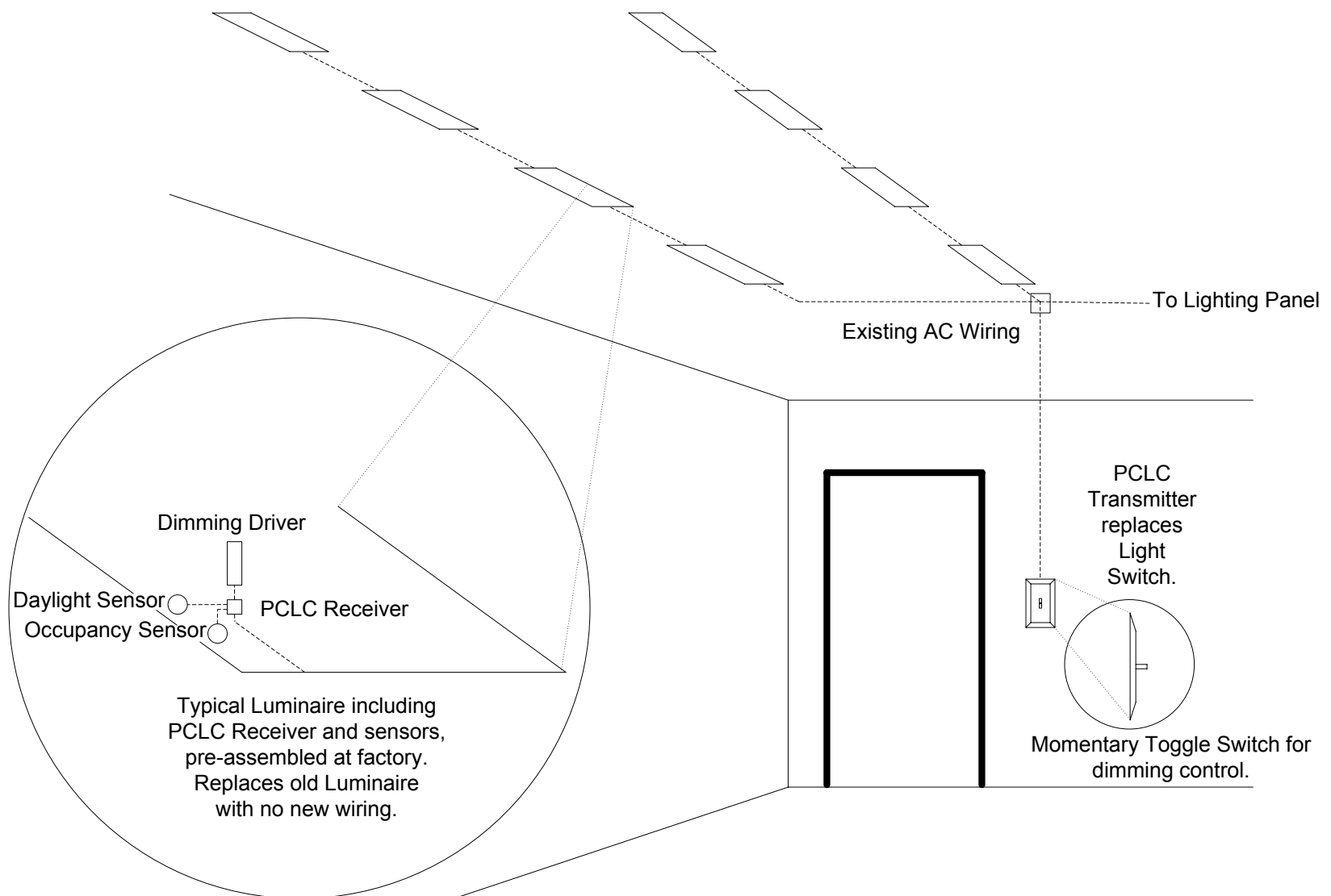
POWERLINE COMMUNICATED LOAD CONTROL Retrofit Room Controller example
